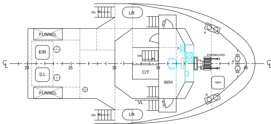
BRIDGE DECK
