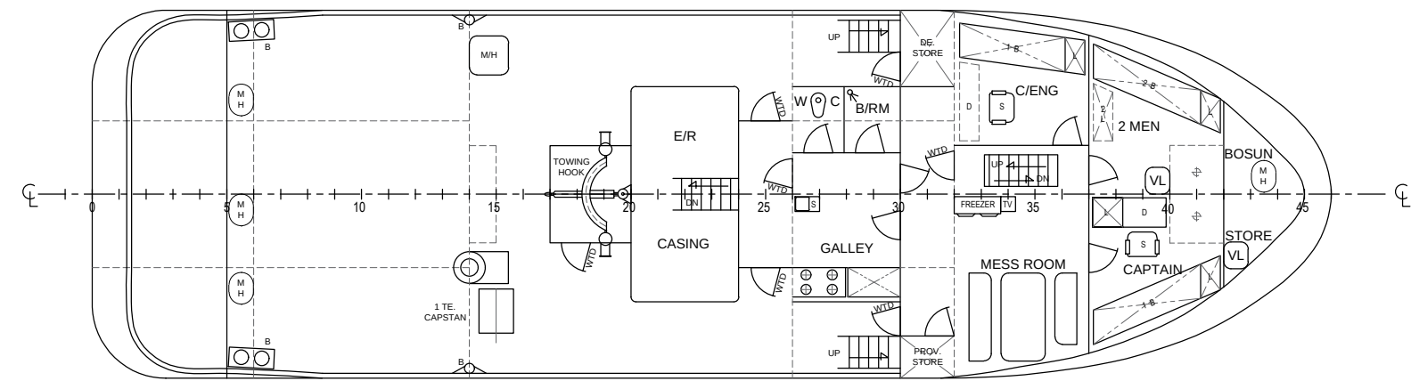
MAIN DECK
