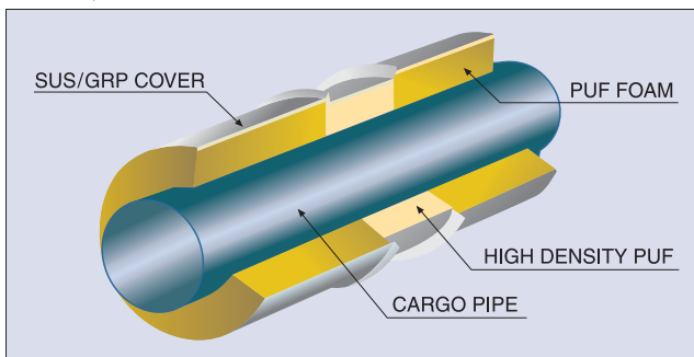
Insulation Construction
