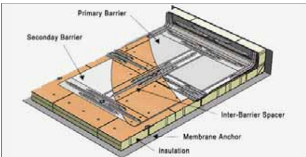
KC-1 Insulation System
