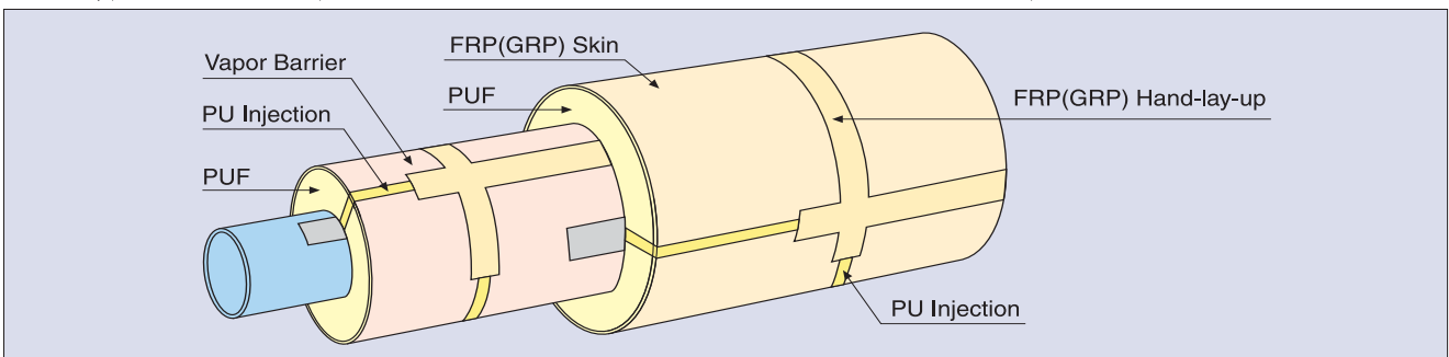
Insulation Construction
