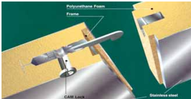
Easy Assembling at Site by Cam Lock System
