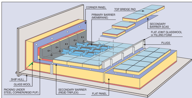
Mark III Insulation System
