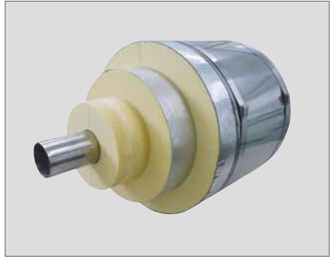
PIR/PUR Pipe Cover with SUS Jacketing
